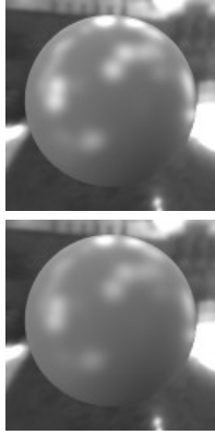
physical sliders
