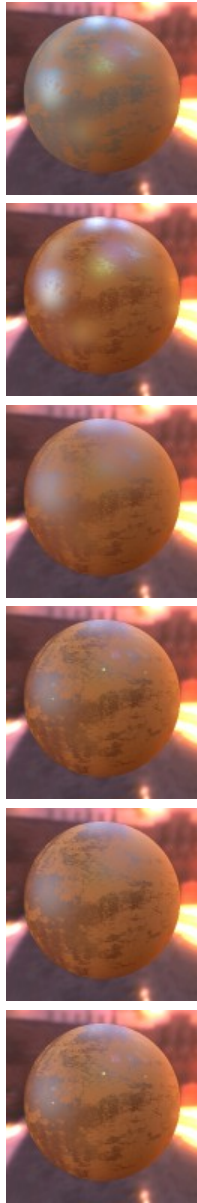
perceptual sliders
