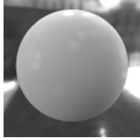
physical sliders
