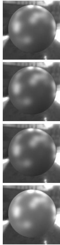
image navigation
