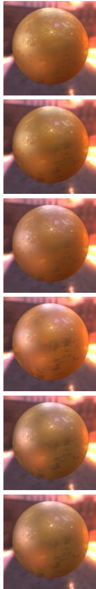
physical sliders
