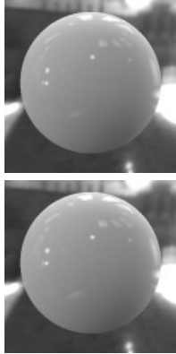
physical sliders
