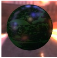
physical sliders
