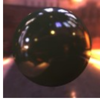
perceptual sliders
