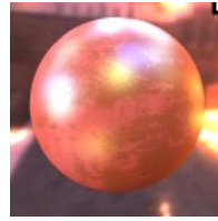
image navigation
