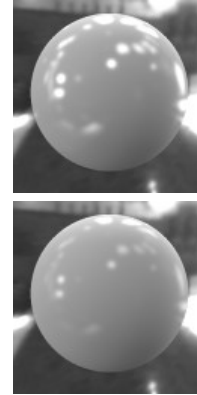
image navigation
