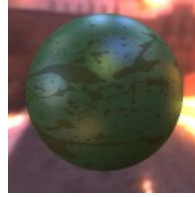
image navigation
