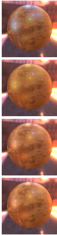
perceptual sliders
