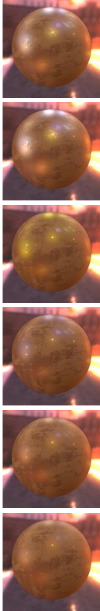
physical sliders
