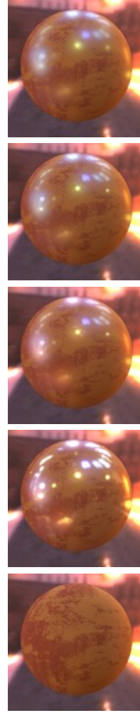
image navigation
