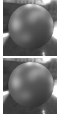
image navigation
