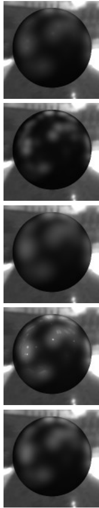
physical sliders
