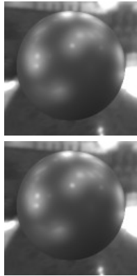
perceptual sliders
